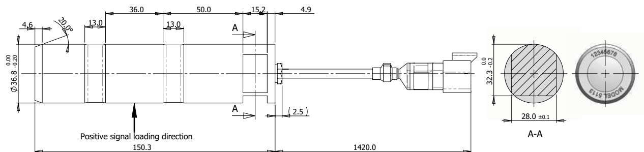
Drawing showing standard connector DT04-3P.
