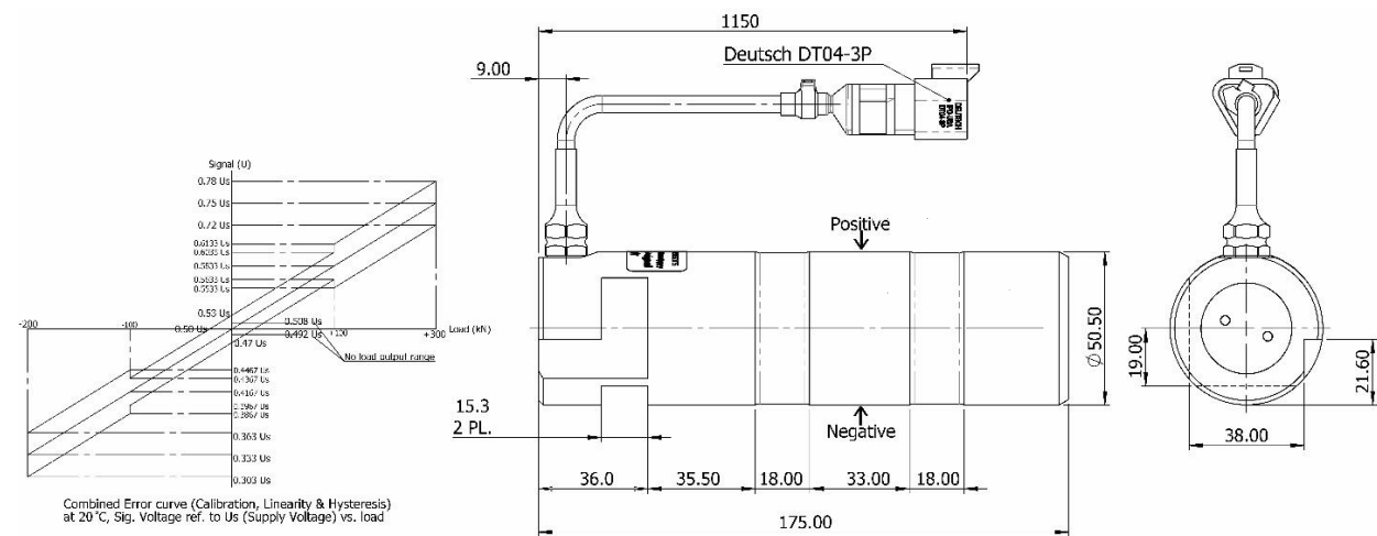
Drawing showing standard connector DT04-3P.
