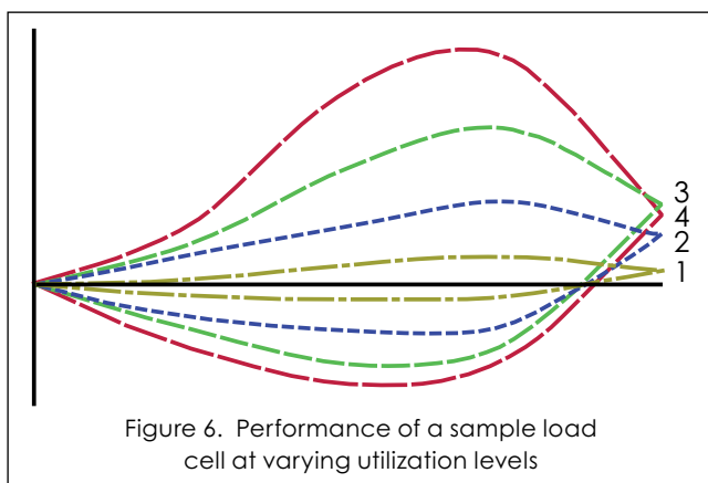
Figure 6 represents the combined error performance of a sample load cell with a rated capacity of 500 kg. The cell has been measured with a utilization of 20% (1), 40% (2), 60% (3) and 80% (4) of the rated capacity.
